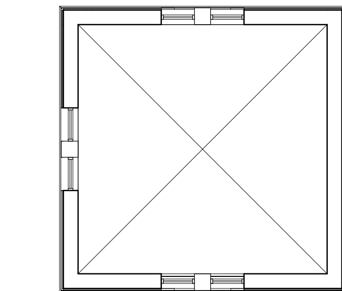
REFLECTED CEILING PLAN - TOWER 2 SCALE: 1/8" = 1'-0" A2.53
